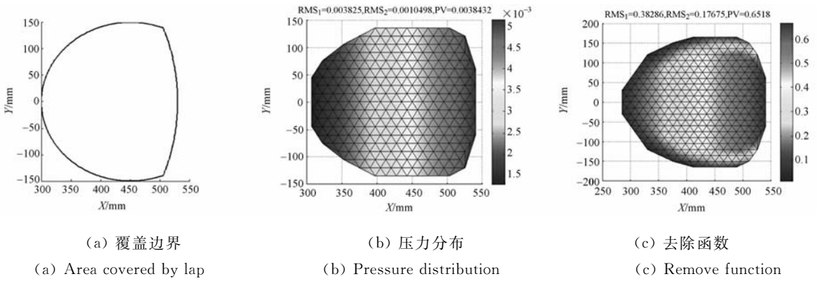
图 5 磨头处于图 3(450, 0)位置时的计算结果 Fig. 5 Calculation results when lap is at (450, 0) in Fig. 3
